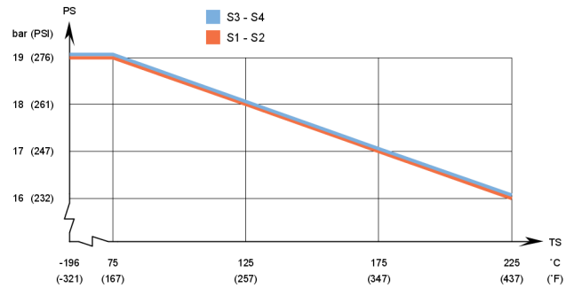
AlfaNova 400AQ – PED approval pressure/temperature graph 1)
